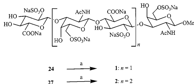
Scheme 6. Catalytic hydrogenation afforded target compounds 1 and 2 ; reagents and conditions: a, H_2 , 10% Pd/C, MeOH/water ( 1 : 93%; 2 : 68%)
