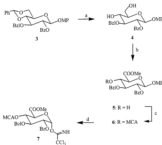
Scheme 1. Synthesis of donor 7 (MCA = monochloroacetyl); reagents and conditions: a, AcOH 60%, 100 °C (85%); b, TEMPO, Aliquat 336, aq. KBr, NaHCO 3 , Ca(ClO) 2 , CH 2 Cl 2 , 0 °C; then MeI, DMF, 50 °C (74%); c, chloroacetic anhydride, pyridine/CH 2 Cl 2 , 0 °C (84%); d, CAN, toluene/MeCN/water; then CCl 3 CN, DBU, CH 2 Cl 2 , 0 °C (70%)
