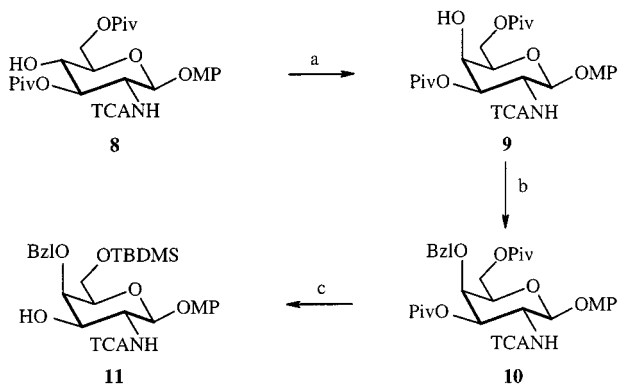
Scheme 2. Synthesis of acceptor 11 (TCA = trichloroacetyl); reagents and conditions: a, \text{Ti}_2\text{O} , pyridine/ \text{CH}_2\text{Cl}_2 , -15 °C to room temp.; then \text{NaNO}_2 , DMF (60%); b, \text{PhCH}_2\text{Br} , \text{Bu}_4\text{NI} , \text{NaH} , THF, 0 °C to room temp. (68%); c, \text{NaOMe} , \text{MeOH} ; then \text{TBDMSCl} , imidazole, DMF, 0 °C (85%)
