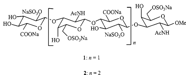
Figure 1. Synthetic chondroitin sulfate D oligosaccharides 1 and 2
