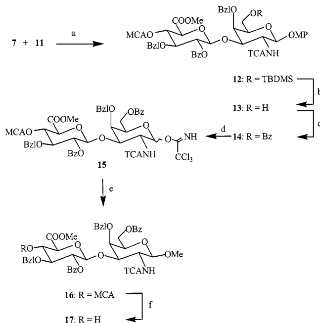
Scheme 3. Synthesis and methyl glycosylation of the key intermediate 15 ; reagents and conditions: a, \text{TMSOTf} , \text{CH}_2\text{Cl}_2 (71%); b, 85% \text{HCOOH} , THF (91%); c, \text{BzCl} , pyridine/ \text{CH}_2\text{Cl}_2 , 0 °C (89%); d, \text{CAN} , toluene/ \text{MeCN} /water; then \text{CCl}_3\text{CN} , \text{DBU} , \text{CH}_2\text{Cl}_2 , 0 °C (64%); e, \text{MeOH} , \text{TMSOTf} , \text{CH}_2\text{Cl}_2 (86%); f, thiourea, pyridine/ \text{EtOH} , 80 °C (91%)
