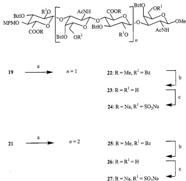
Scheme 5. Preparation of protected O -sulfonated oligosaccharides 24 and 27 ; reagents and conditions: a, Bu 3 SnH, AIBN, NN-di-methylacetamide, 95 °C ( 22 : 68%; 25 : 81%); b, LiOH/H 2 O 2 , THF, 0 °C to room temp.; then 4 M NaOH, MeOH ( 23 : 68%, 26 : 80%); c, Me 3 N.SO 3 , DMF, 50 °C; then ion-exchange resin [Na + ] ( 24 : 67%, 27 : 54%)
