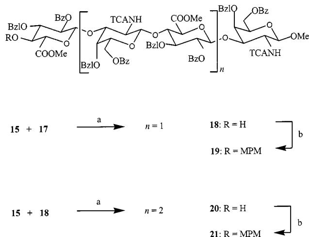
Scheme 4. Syntheses of oligosaccharides 18–21 ; reagents and conditions: a, TMSOTf, CH 2 Cl 2 ; then thiourea, pyridine/EtOH, 80 °C ( 18 : 44%; 20 : 46%); b, 4-methoxybenzyl trichloroacetimidate, TMSOTf, CH 2 Cl 2 , 0 °C ( 19 : 60%; 21 : 70%)
